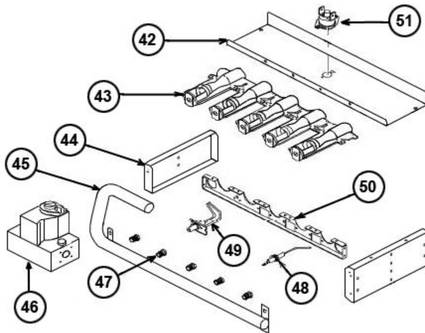
Burner Assembly
