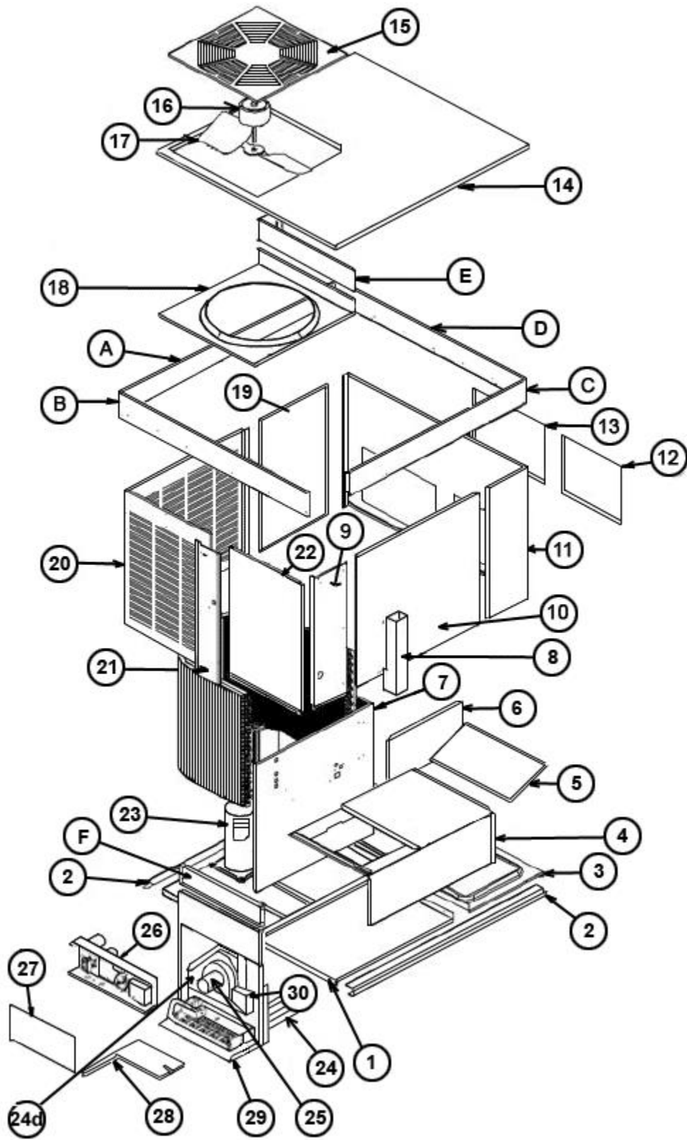
Exploded View
