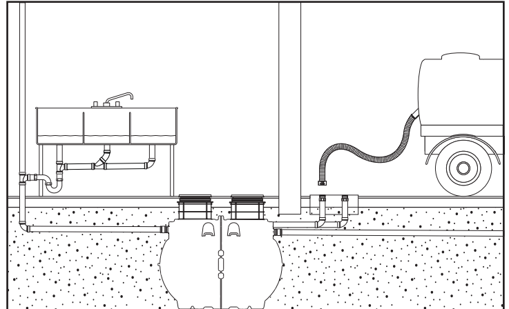
Below Grade Installation with Outdoor In-Ground Remote Pumpout Hook-up
