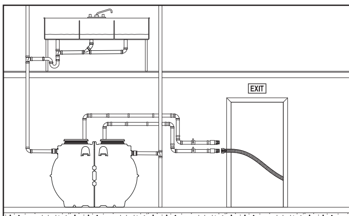
At Grade Floor Below Installation with Indoor Remote Pumpout Hook-up
