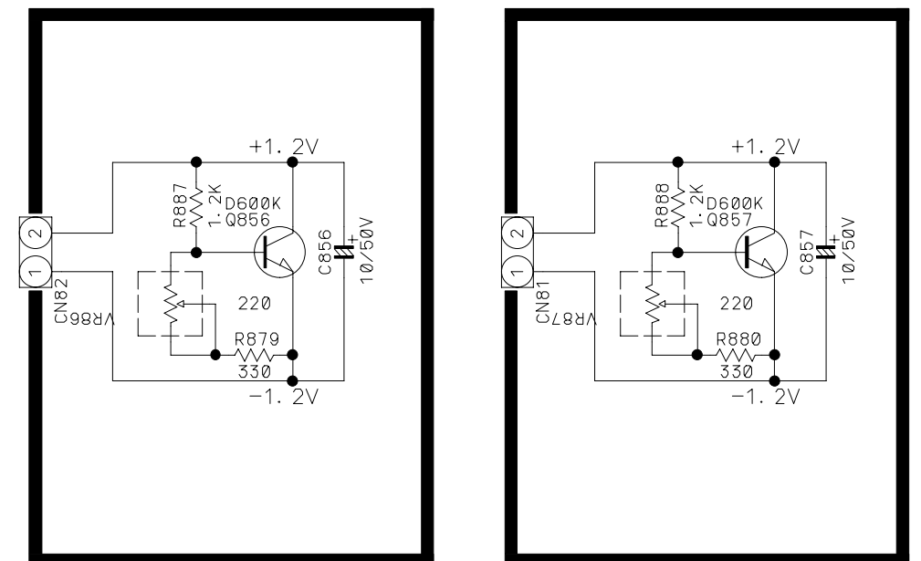
MAIN BOARD 2 (BIAS & REGULATOR)
