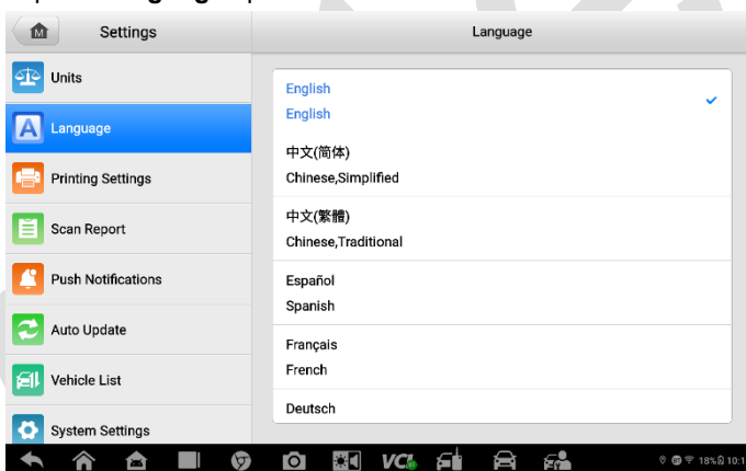
Figure 9-2 Language Screen
