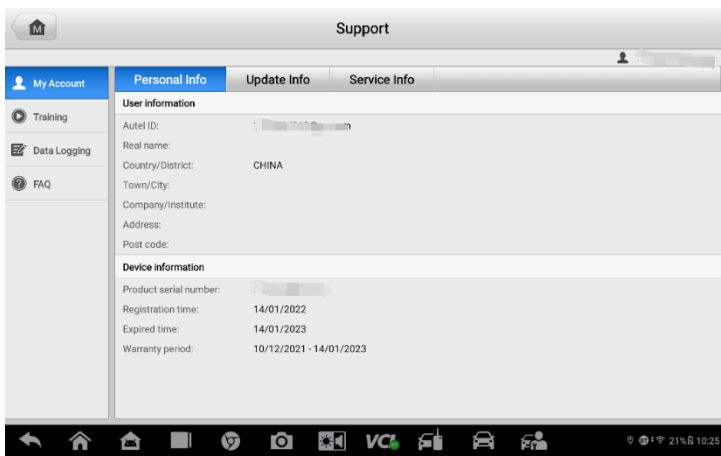
Figure 12-1 Support Screen
