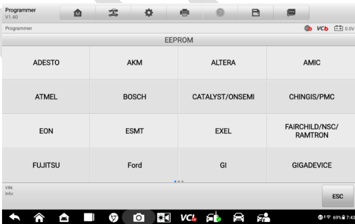
Figure 5-3 EEPROM Screen
