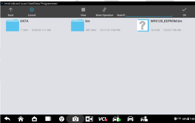
Figure 5-7 Write Screen
