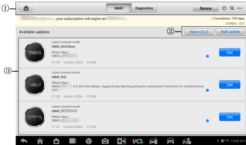
Figure 8-1 Update Screen
