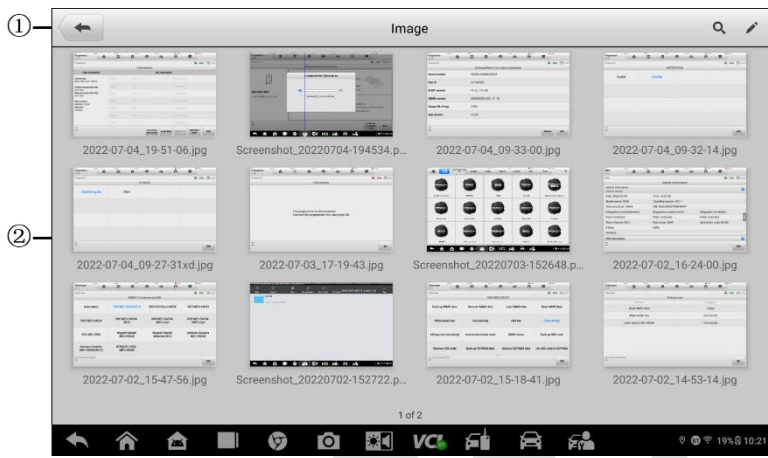
Figure 11-4 Image Screen
