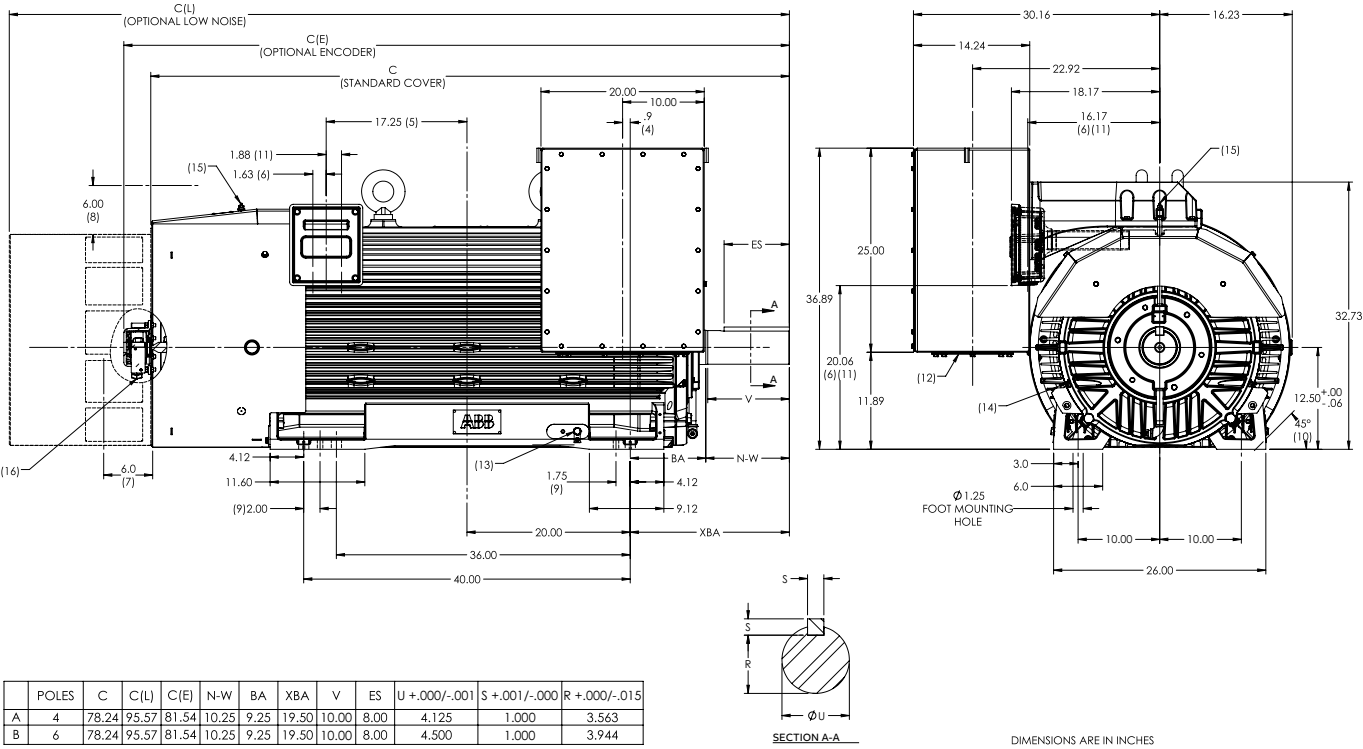
Squirrel-cage induction motors, frame NXR US 5012, terminal box mounting F1
