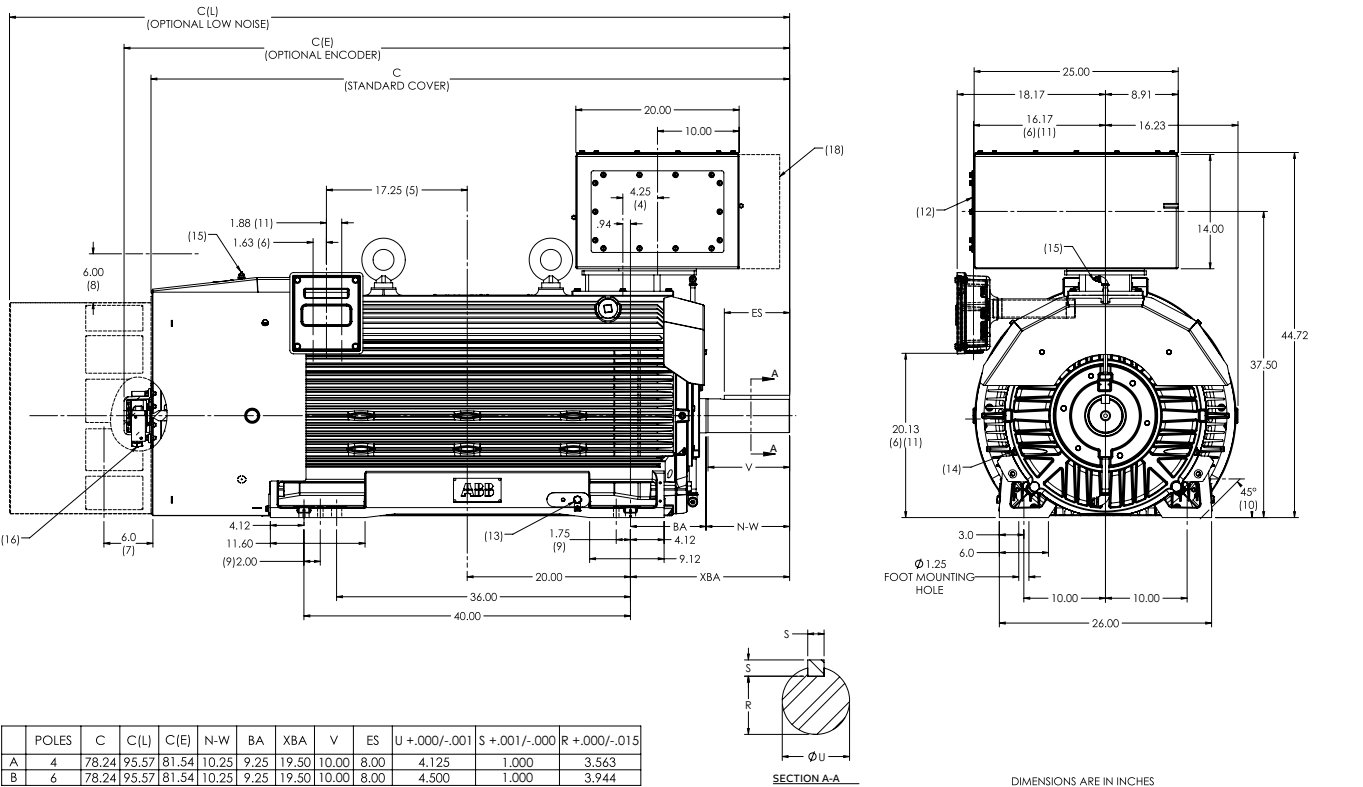
Squirrel-cage induction motors, frame NXR US 5012, terminal box mounting F3
