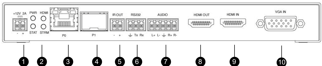
FIG. 1 N2312 Encoder Front Panel
