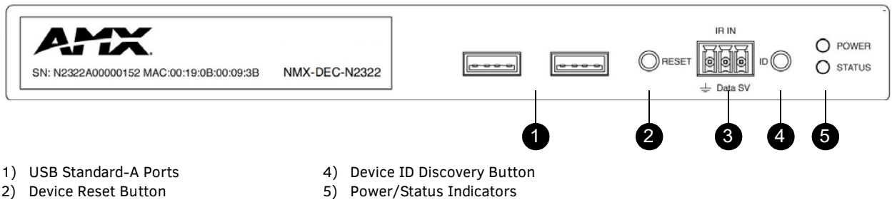
FIG. 3 N2322 Decoder Front Panel
