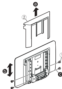
① Stelschroef (4 mm × 6 mm) ② Monitorafdekking
