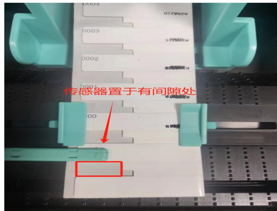
Sensor place on the label gap
