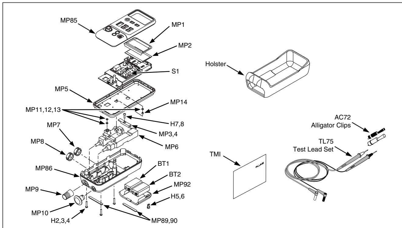
Figure 9. Replacement Parts
