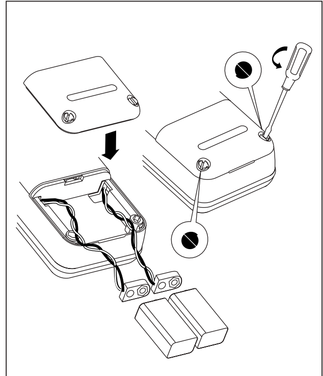
Figure 8. Battery Replacement
