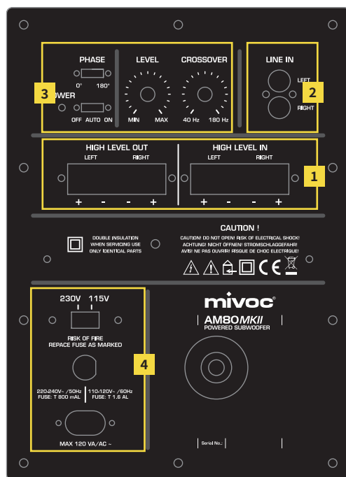
Figure 2. AM 80MKII – connection terminal
