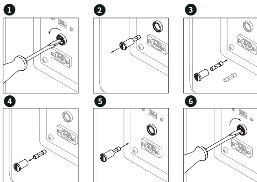
Figure 9. AM 80MKII – Changing fuses
