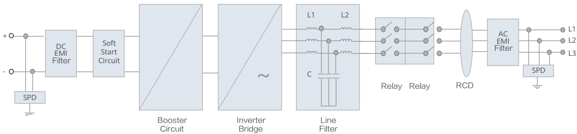
LUNA2000-213KTL
