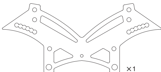
碳纖維前避震板 Carbon front damper stay 210298
