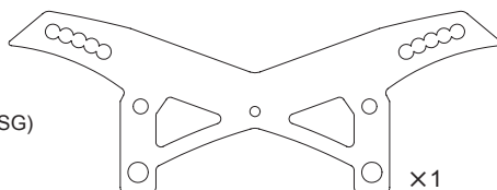
碳纖維前避震板 Carbon front damper stay 210298
