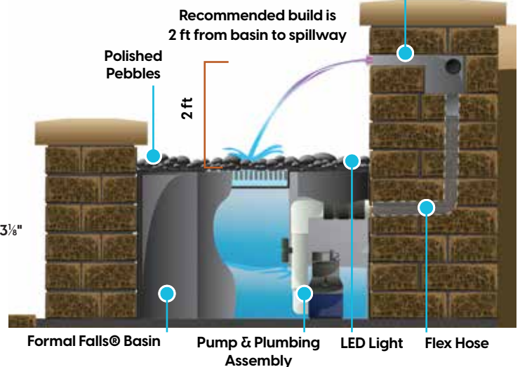
Formal Falls Side View Cutaway Diagram
