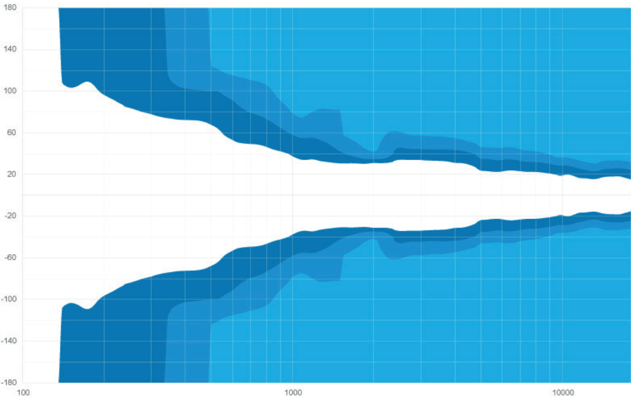
VENU 8ix Vertical beamwidth
