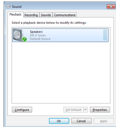
Windows 7 screen
