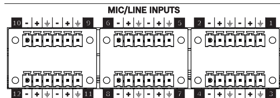
Figure 5.1: Analog input connections
