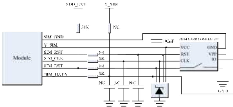
Figure 3.12:Reference design drawing of the card holder with hot-swappable function
