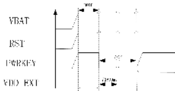
Figure 3.7: Boot sequence diagram
