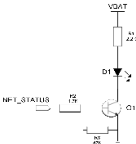
Figure 3.17:NET_STATUS reference circuit
