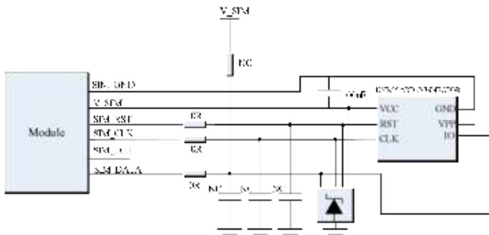
Figure 3.13:Reference design drawing of deck without hot-swappable function
