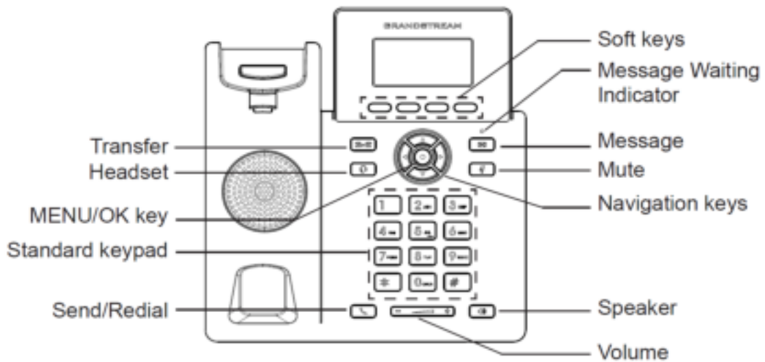
Figure 6: GRP2601 Keyboard
