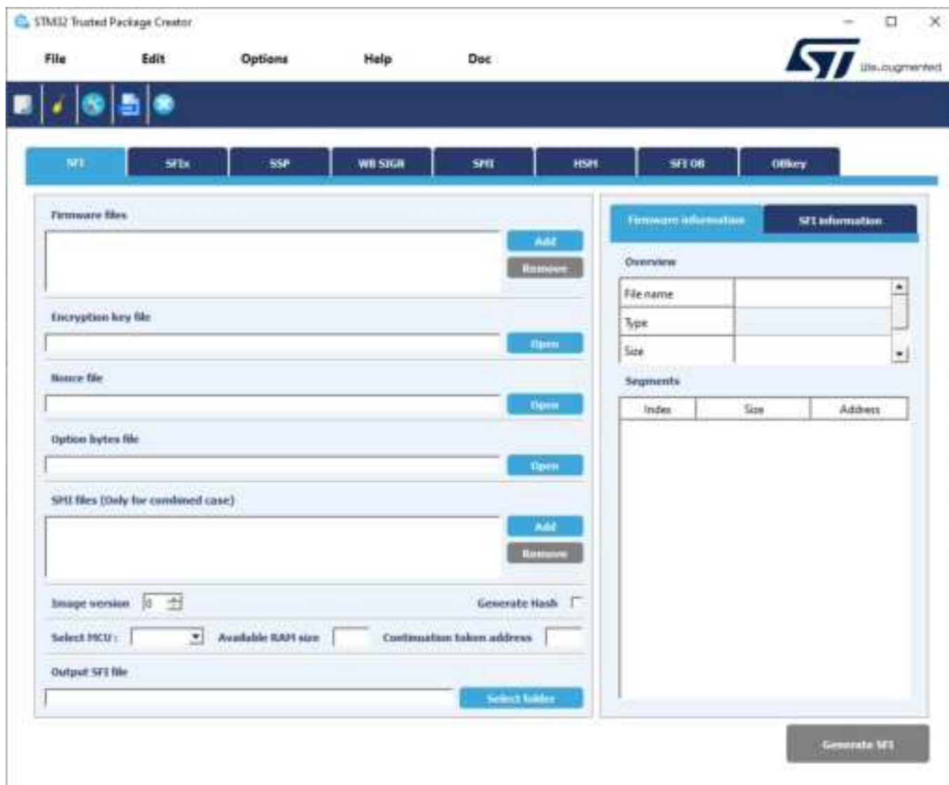
Figure 14. STM32 Trusted Package Creator - SFI image creation
