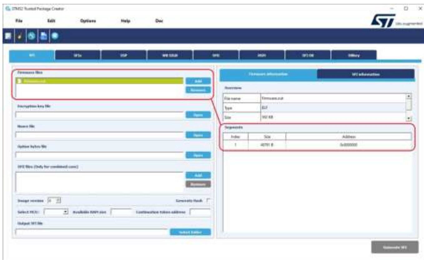
Figure 16. SFI image generation tab example
