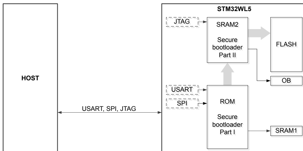
Figure 12. STM32WL5 secure bootloader
