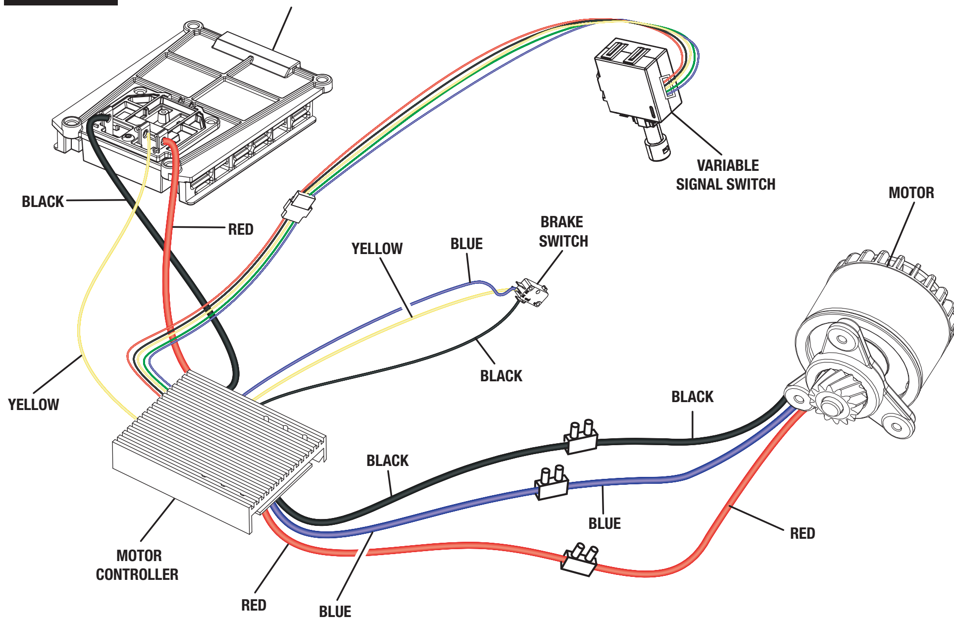
WIRING DIAGRAM
