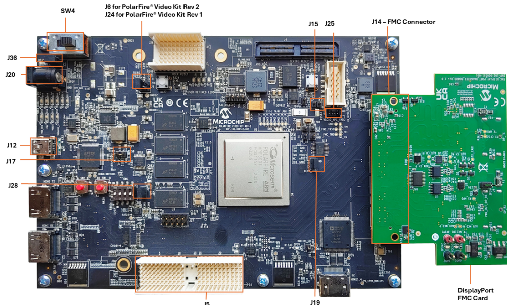
Figure 3-1. Setting up the Hardware
