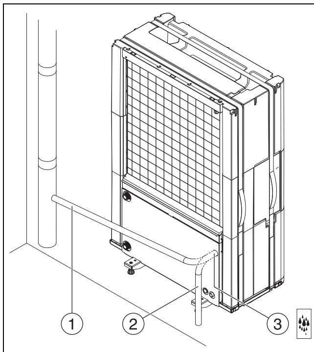
Fig. 17 Condensate tube connections, valid for all sizes
