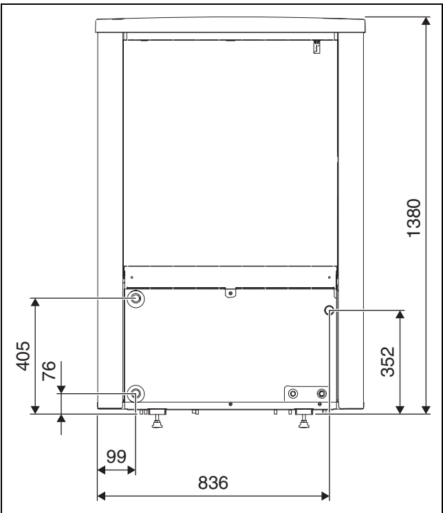
Fig. 4 Dimensions and connections of heat pump models 5 OR-S-9 OR-S
