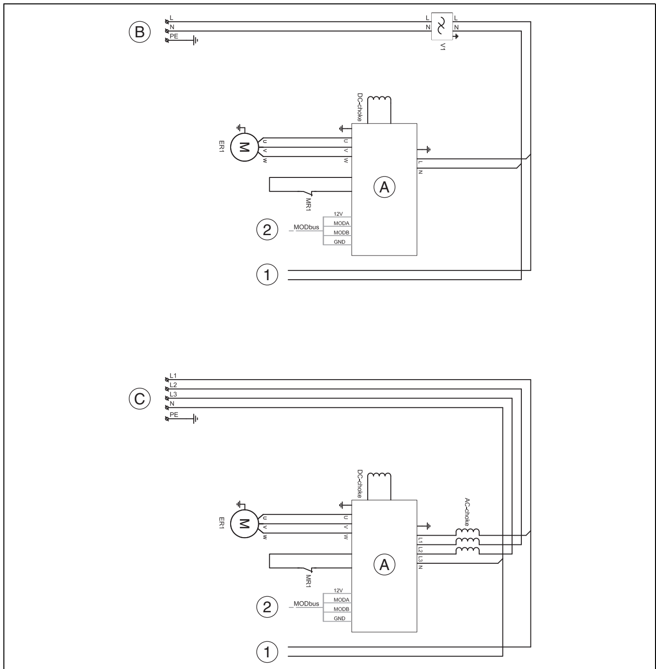
Fig. 25 Wiring diagram for transformer, alternating current / three-phase current
