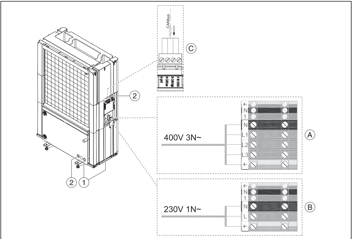
Fig. 20 Cable conduits and control device
