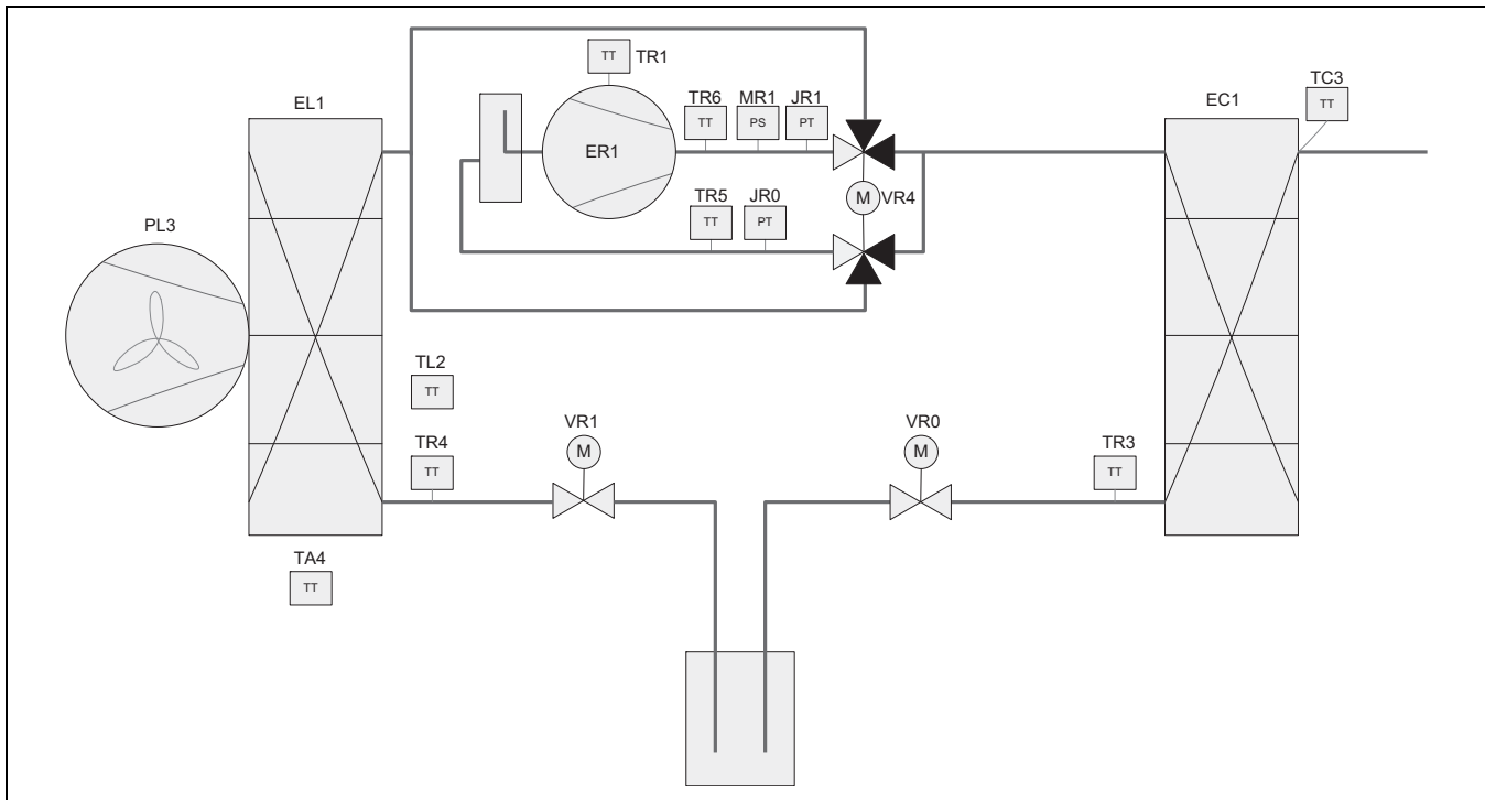
Fig. 24 Refrigerant circuit
