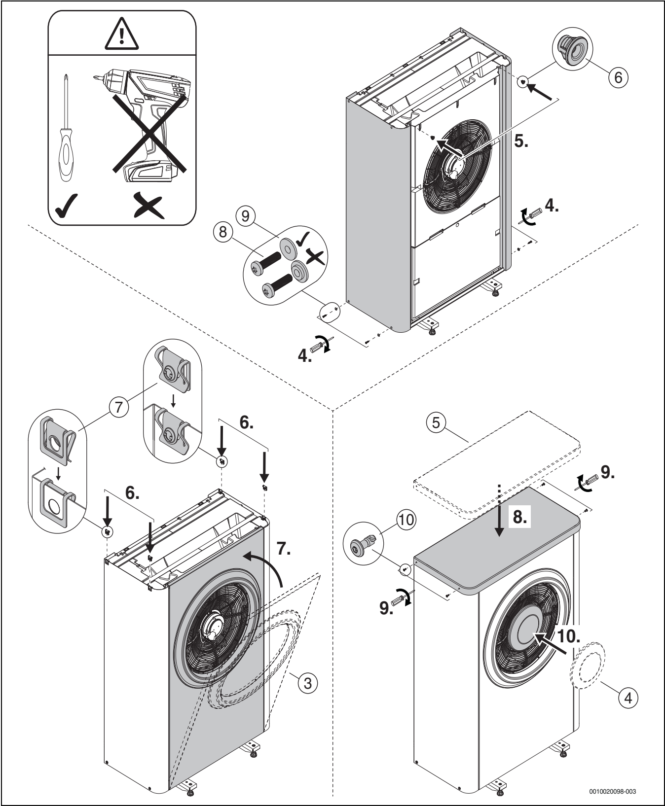
Fig. 22 Installing side panels and cover
