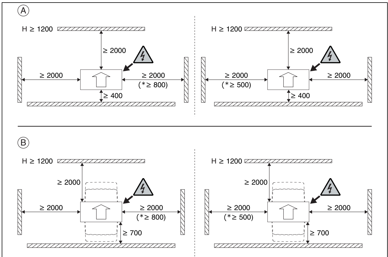
Fig. 8 Clearances during setup
