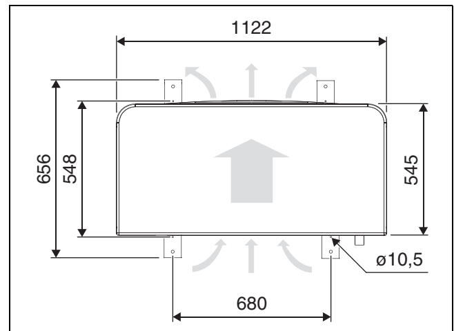
Fig. 7 Dimensions of heat pump models 13 OR-S-17 OR-T, view from top
