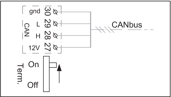
Fig. 19 Termination CAN-BUS
