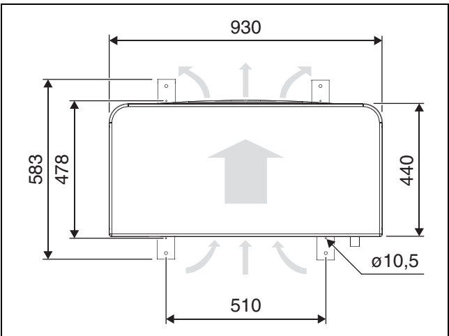
Fig. 5 Dimensions of heat pump models 5 OR-S-9 OR-S, view from top
