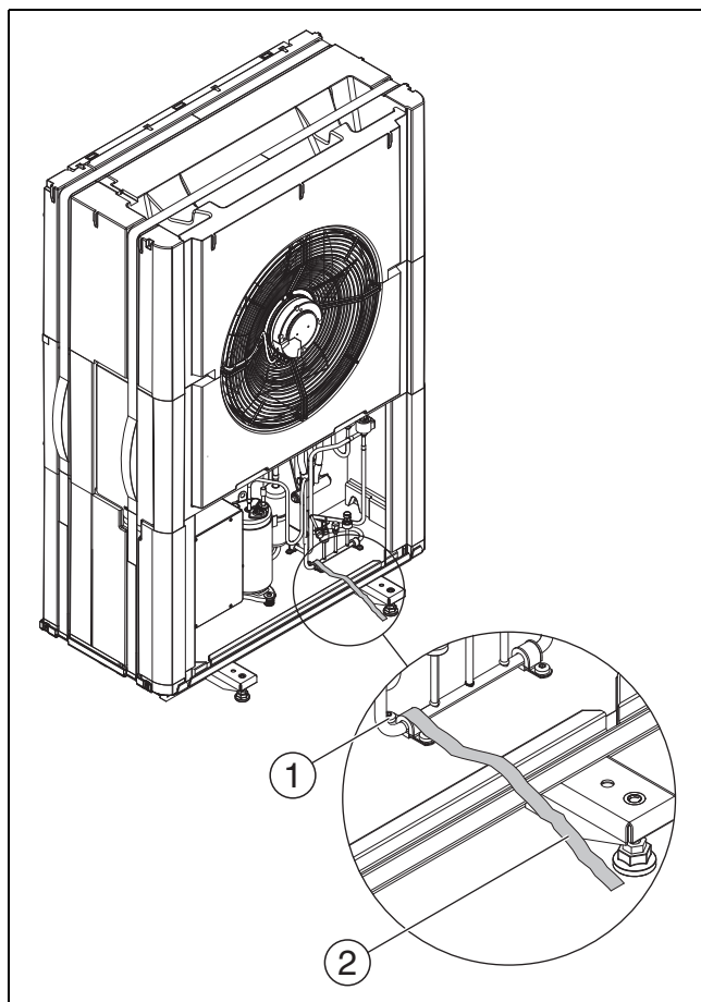
Fig. 13 Transport fitting
