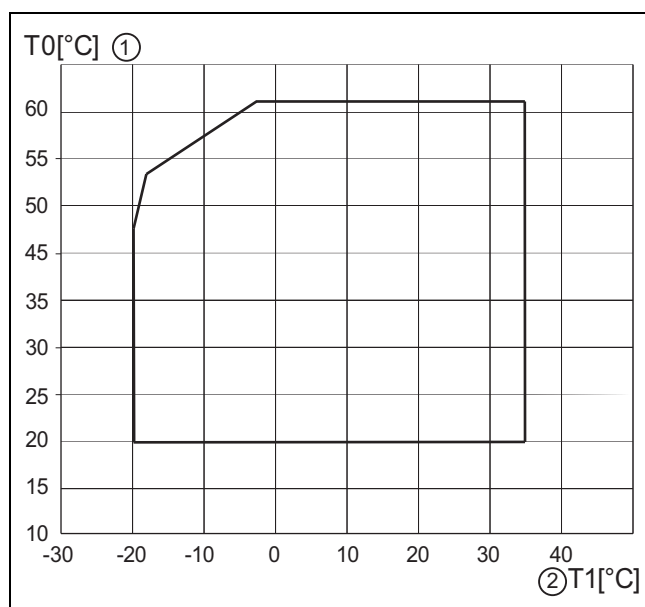
Fig. 23 Heat pump without auxiliary heater
