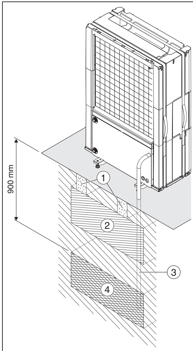
Fig. 12 Condensate pipe in gravel bed
