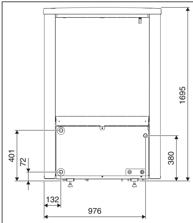
Fig. 6 Dimensions and connections of heat pump models 13 OR-S-17 OR-T
