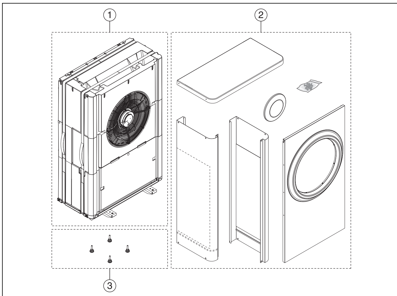
Fig. 2 Supplied parts
