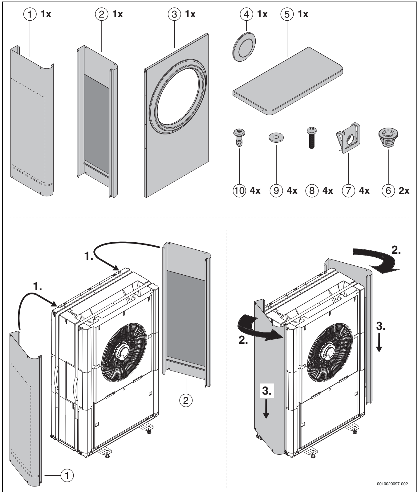
Fig. 21 Installing side panels and cover
