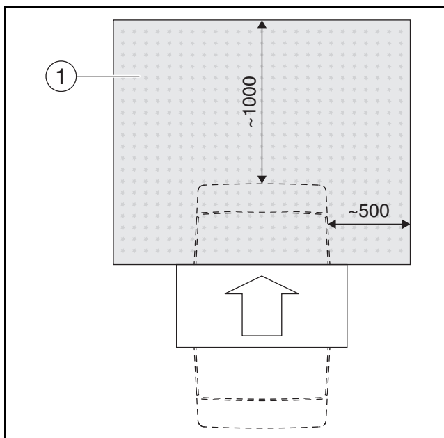
Fig. 11 Danger! Ice formation in front of the heat pump with sound hood (accessory)
