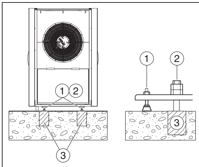
Fig. 14 Fastening the heat pump
