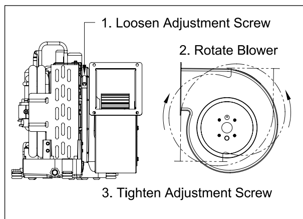
FIGURE 2. Blower rotation
