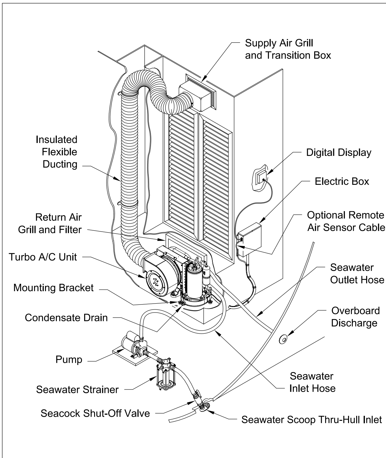
FIGURE 1. Installation overview
