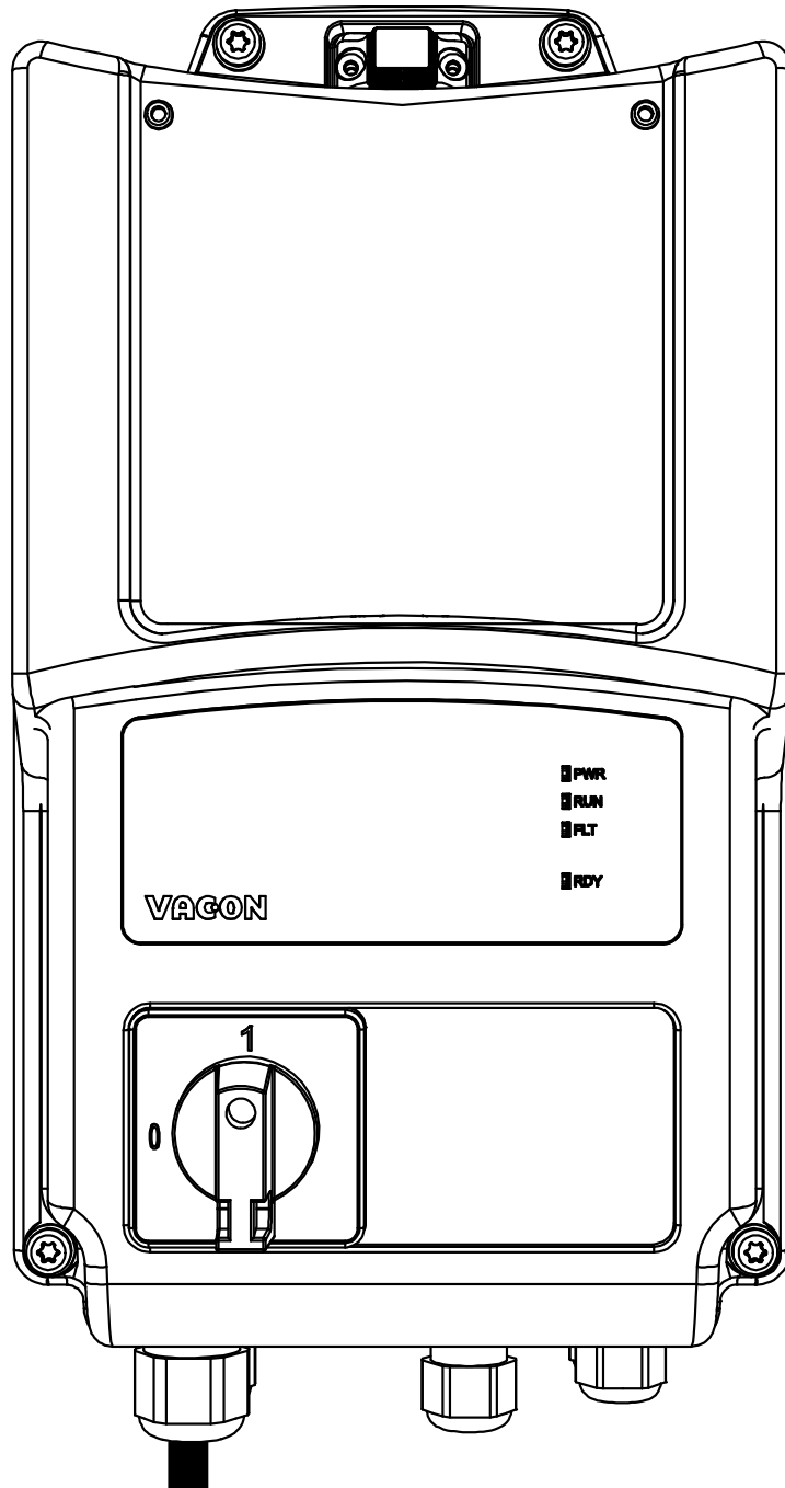
Figure 4. Mount the plastic cover.
