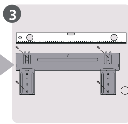
Attach Mounting Plate
