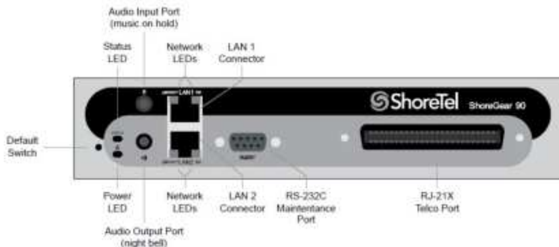
Figure 38: SG90 Front Plate
