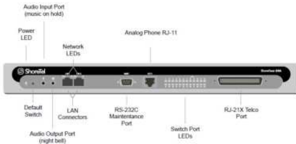
Figure 53: SG24A Front Plate
