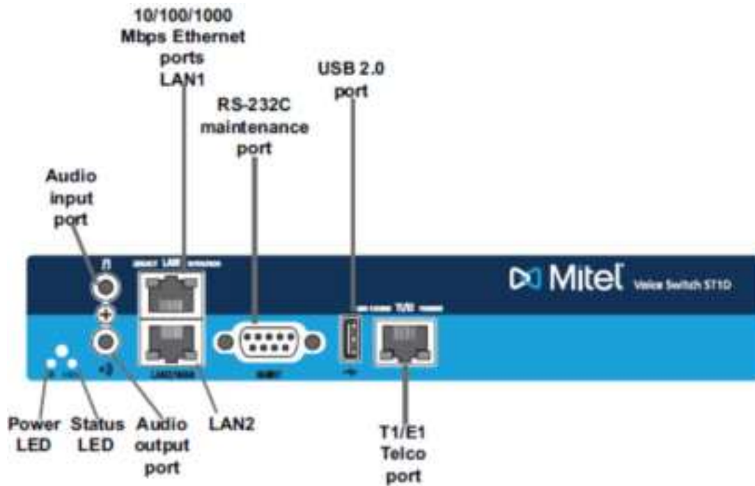
Figure 31: Voice Switch ST1D Front Plate
