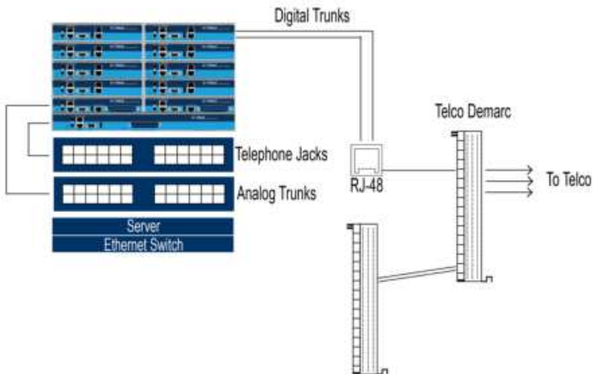
Figure 21: Rack Installation
