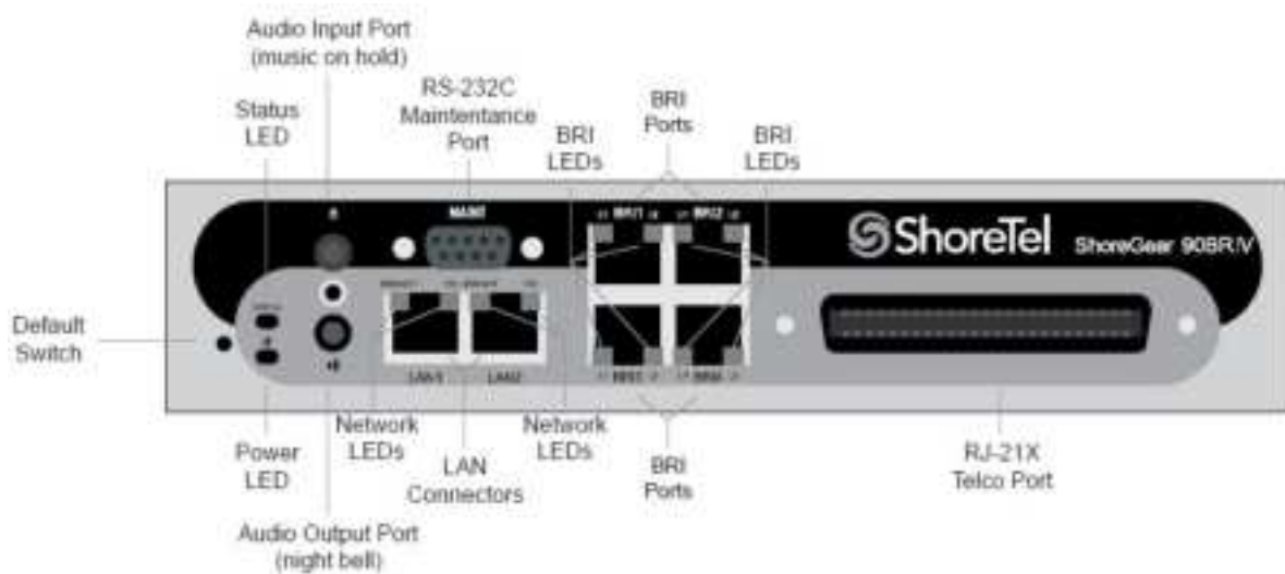
Figure 39: SG90BRI Front Plate
