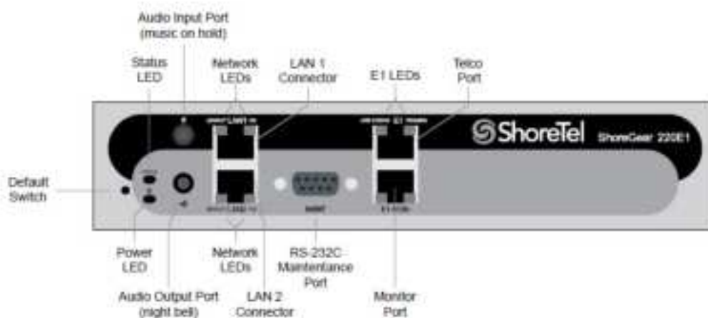
Figure 45: SG220E1 Front Plate
