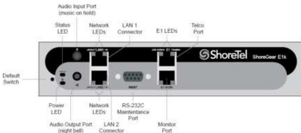
Figure 47: SGE1k Front Plate
