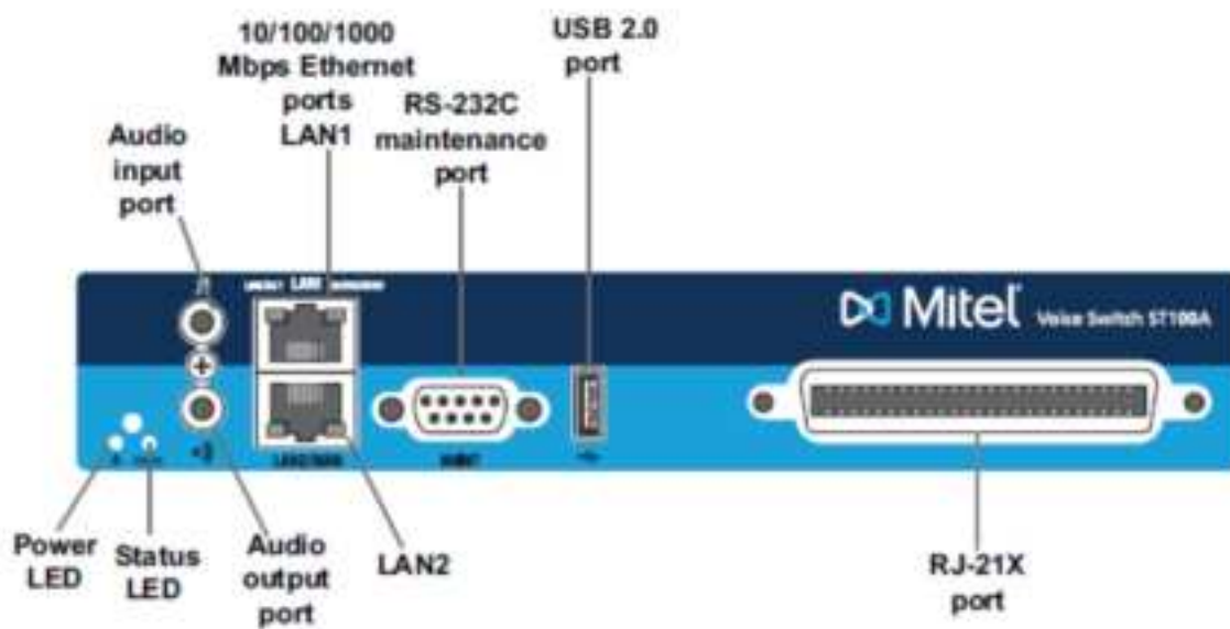
Figure 34: Voice Switch ST100A Front Plate
