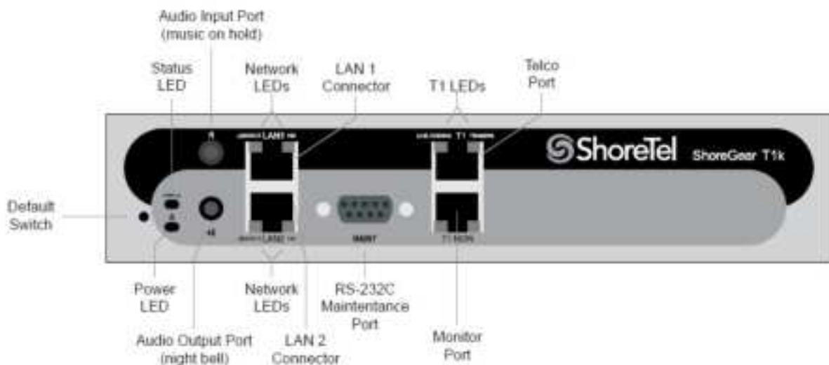
Figure 46: SGT1k Front Plate
