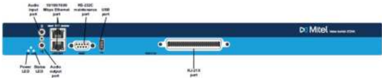
Figure 51: Voice Switch ST24A Front Plate
