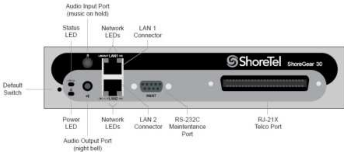
Figure 41: SG30 Front Plate
