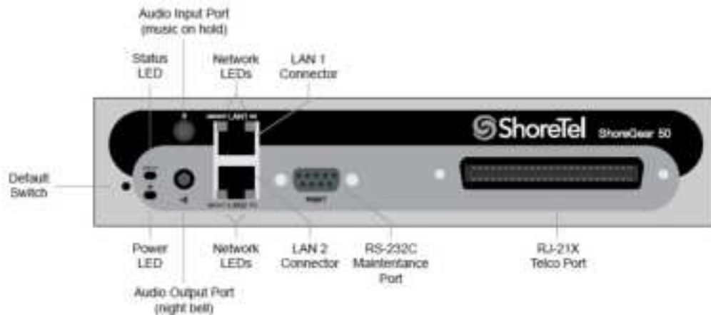
Figure 40: SG50 Front Plate
