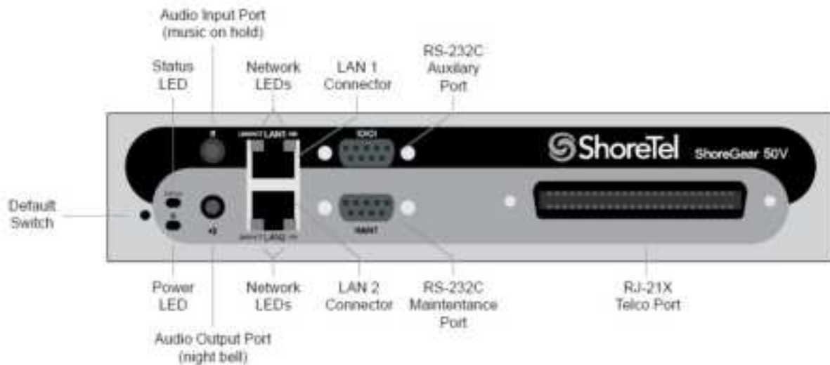
Figure 50: SG50V Front Plate
