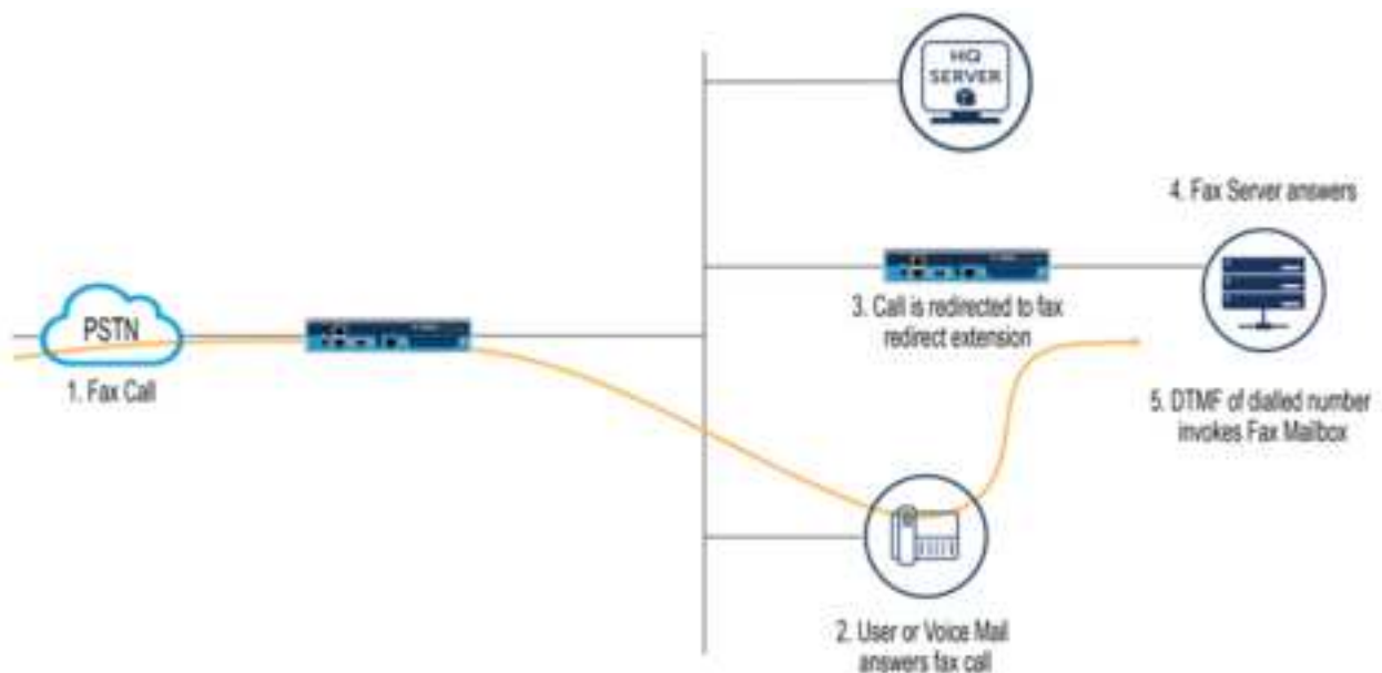
Figure 15: Fax Server Integration Call Flow
