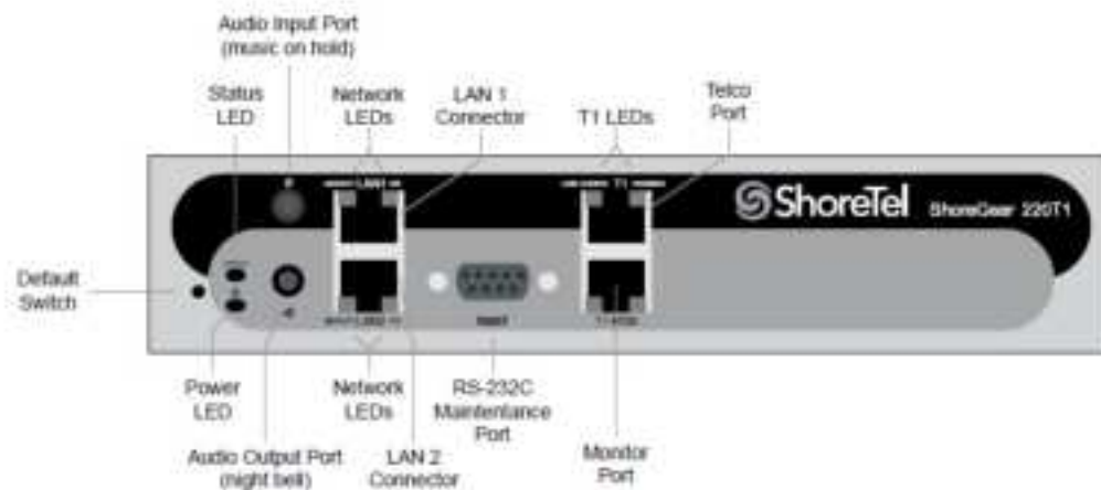
Figure 43: SG220T1 Front Plate
