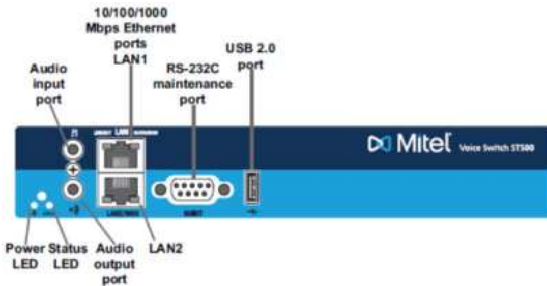
Figure 36: Voice Switch ST500 Front Plate
