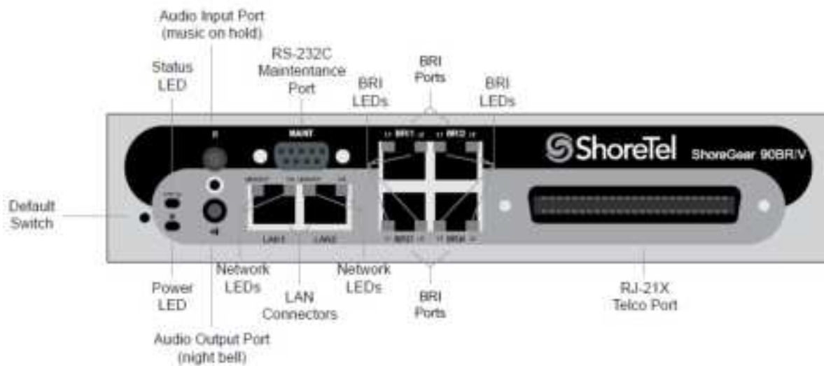
Figure 49: SG90BRIV Front Plate
