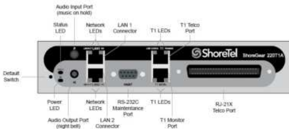
Figure 44: SG220T1A Front Plate
