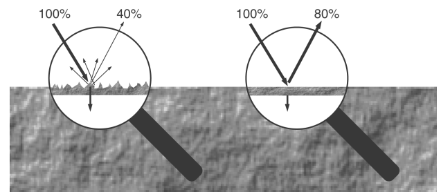
Figure 10: The texture of the material determines how much light is reflected and how much is absorbed Problems caused by shadows from walls or furniture can be solved by ensuring that there are sufficient radiators and that they are well positioned, so that a strong enough infrared field is produced over the whole conference area. Care should be taken not to direct radiators towards uncovered windows, as most of this radiation will subsequently be lost.
