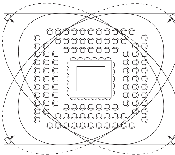
Figure 15: Radiators covering seats arranged in a square
