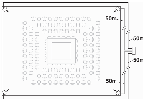
Figure 23: Radiators with equal cable length
