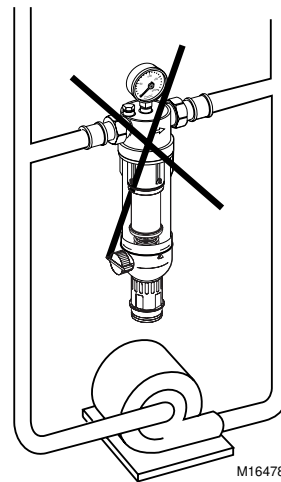
Fig. 2f. Ensure the F76S is not installed in a bypass across a pump.
