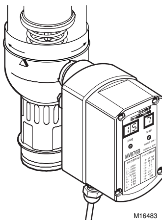
Fig. 6. Final position of MV876 and F76S components.
