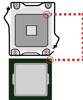
2-4 CPU Installation
