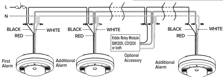
Figure 9-D, Interconnect Wiring Diagram
