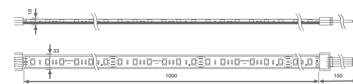
Dimension: LM SV 800 TW DC 48W
