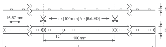
Dimension: LM-SV-900
