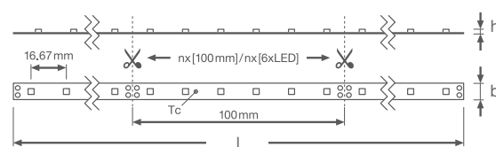
Dimension: LM-SV-900
