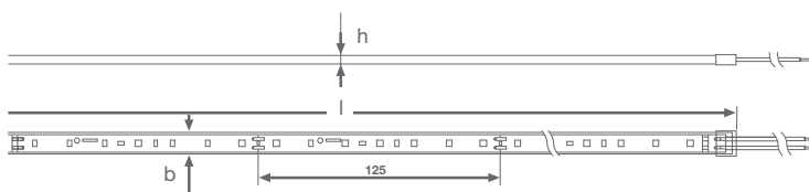
Dimension: LM-SP (1000, 1500 & 2000)
