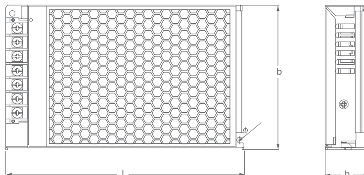
Dimension: LVED VAL 350W 24V (Metal Housing)
