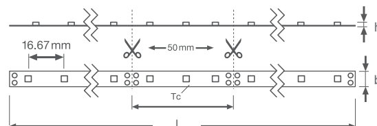
Dimension: LM-SV-900
