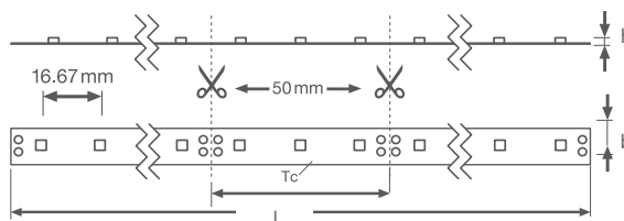
Dimension: LM-SV-900
