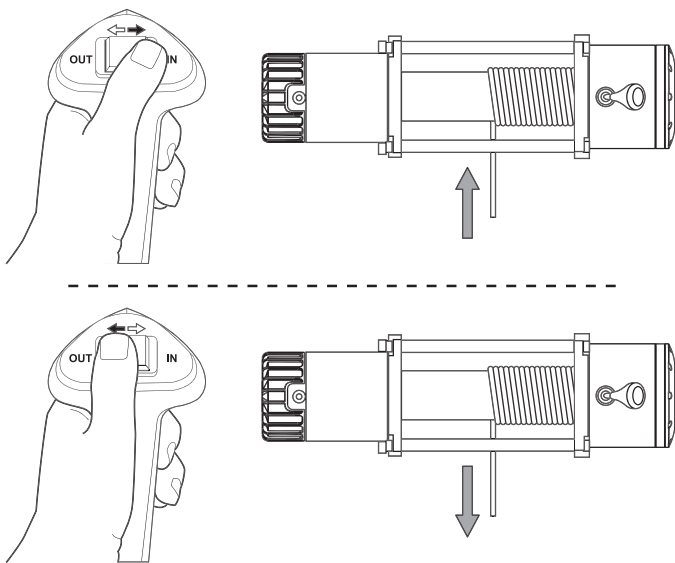
Figure L: Pendant controls
