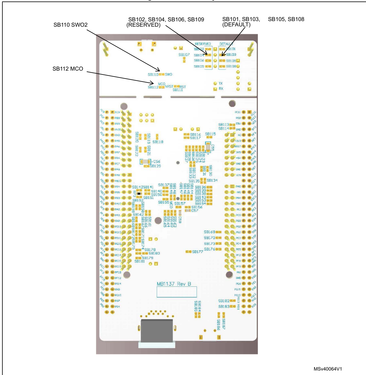
Figure 5. Bottom layout
