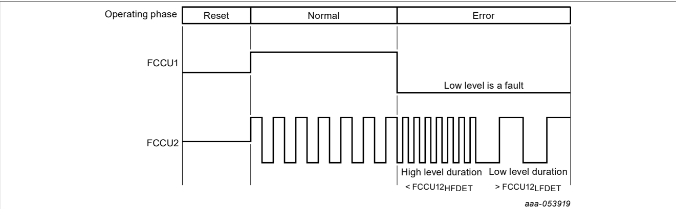
Figure 17. Example of FCCU independent pins reaction upon a fault
