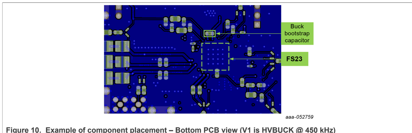
Figure 10. Example of component placement – Bottom PCB view (V1 is HVBUCK @ 450 kHz)
