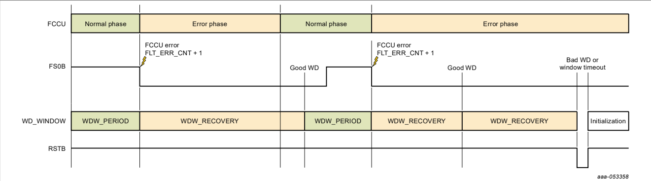
Figure 18. Fault recovery strategy principle
