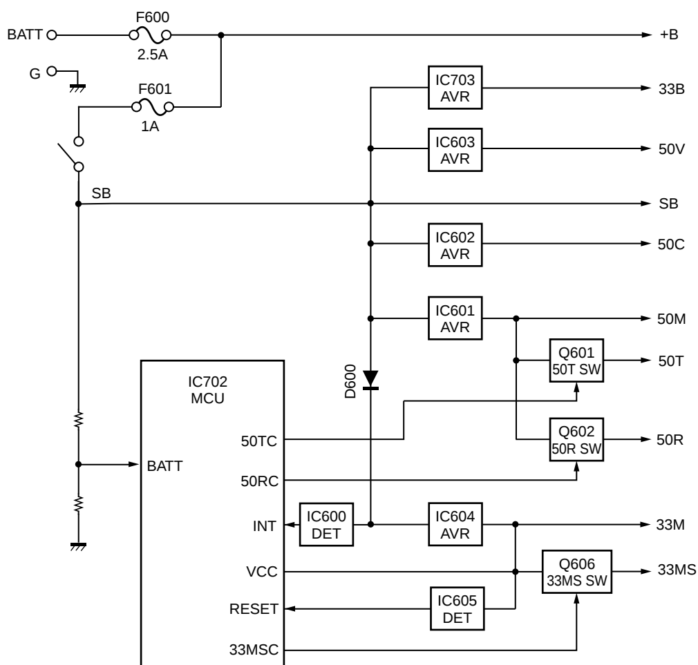
Fig. 9 Power Supply
