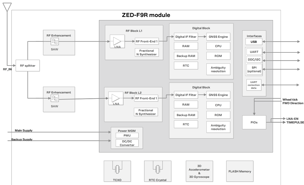
Figure 1: ZED-F9R block diagram
