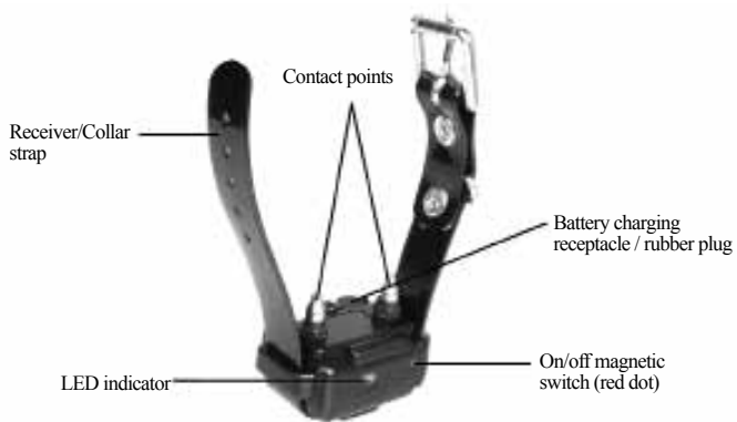
Receiver/Collar
