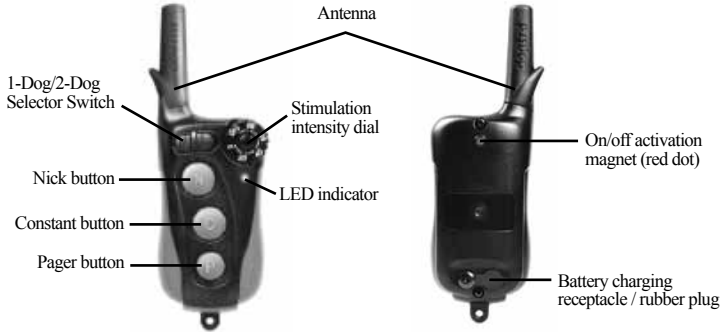
Handheld Transmitter
