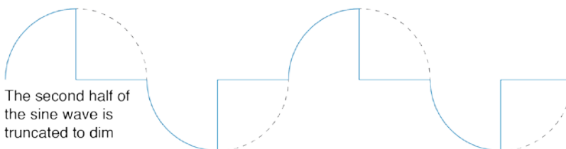
Trailing-Edge Dimmer
