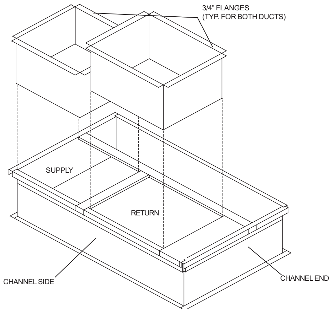
Figure 6. Roof Mounting Curb Field Fabricated (Side X Side) Ducts
