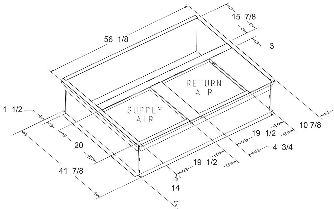
Figure 3. BAYCURB051 Full Perimeter Roof Mounting Curb Outline
