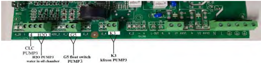
ELETRONIC BOARD B
