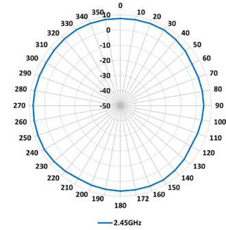
2.4GHz Band - Azimuth
