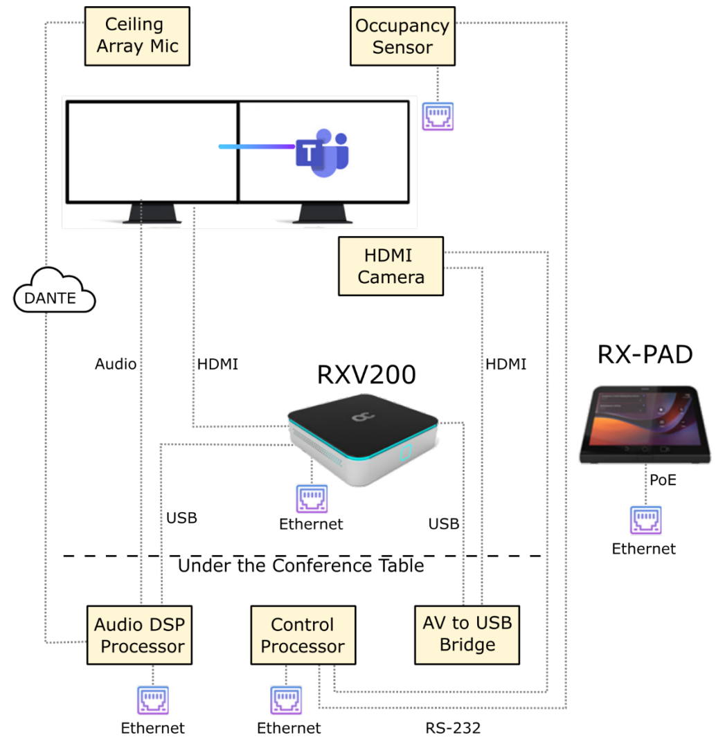
Connection Diagram for RXV200-B05
