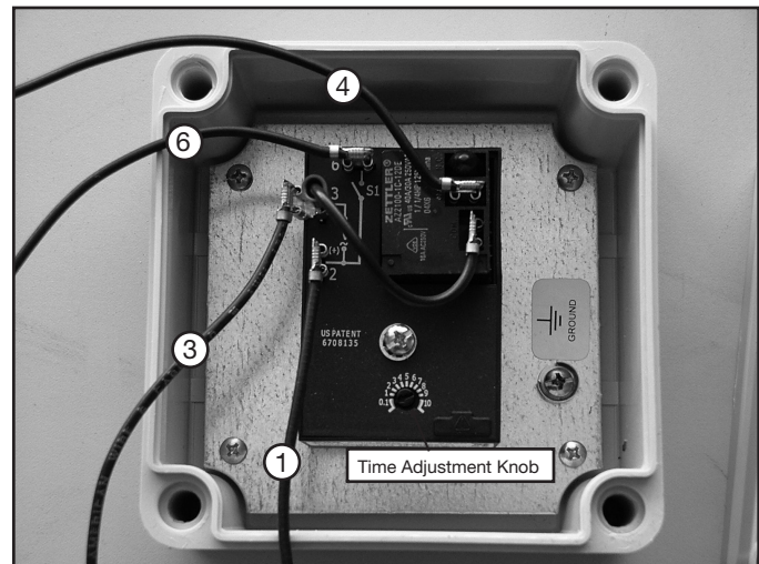
Figure 3. 120V or 208/240V Time Delay Relay
