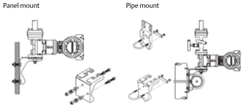
Figure 1-2: Mounting Brackets – Traditional Flange
