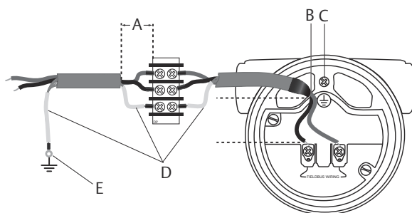
Figure 4-1: Transmitter Wiring
