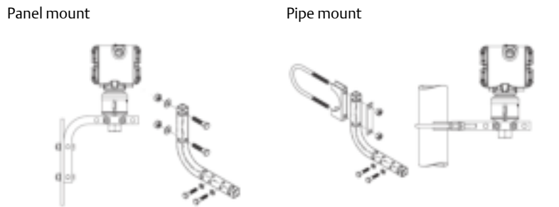
Figure 1-3: Mounting Brackets – In-line
