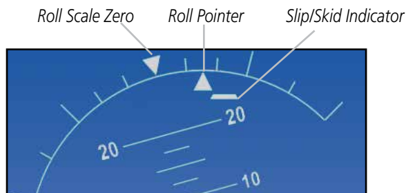
Slip/Skid Indicator
