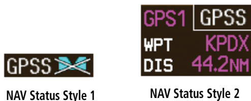
GPSS Mode Annunciations
