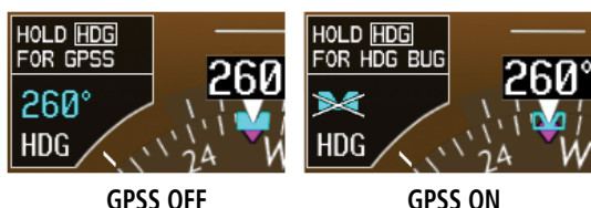
GPSS Mode Control
