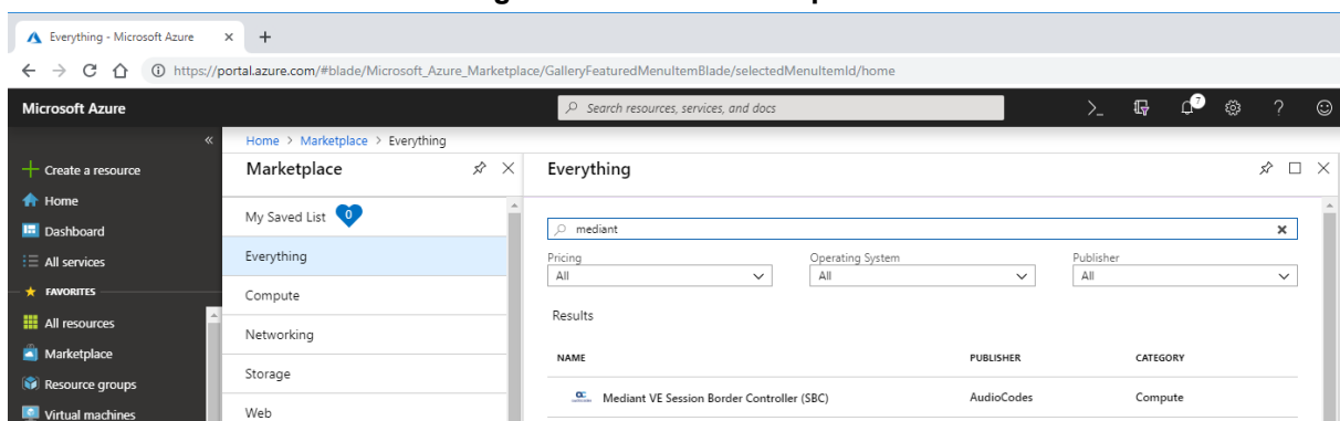
Figure 3-2: Azure Marketplace
