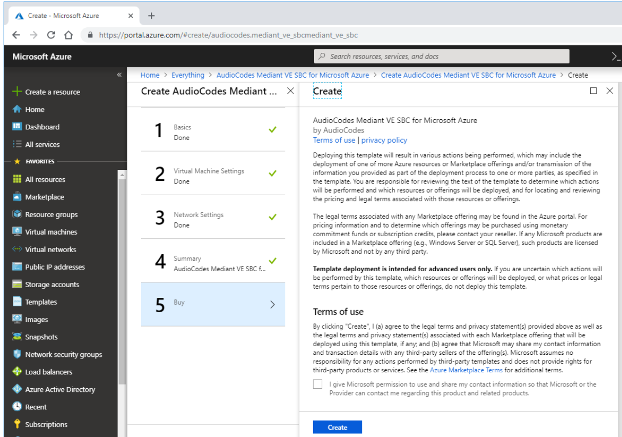
Figure 3-5: Buy Step
