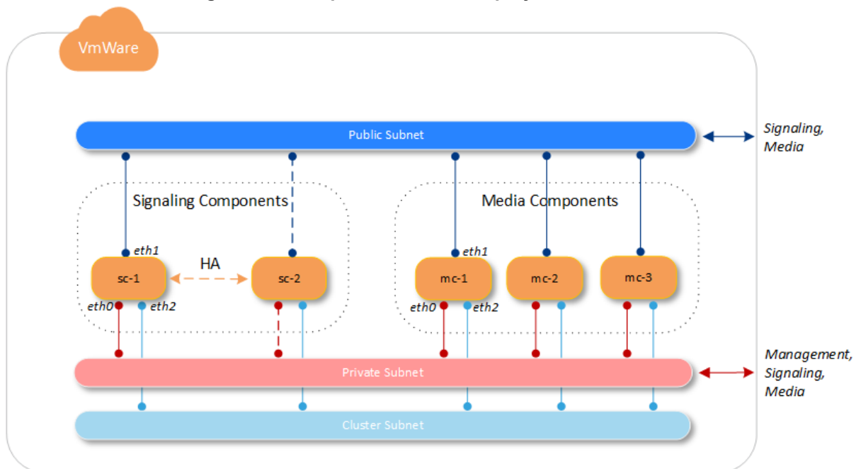
Figure 7-1: Sample Mediant CE Deployment In VMware
