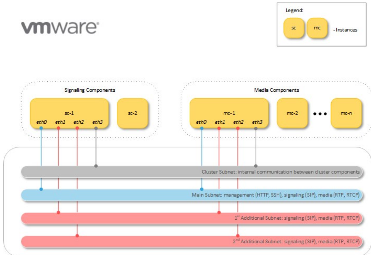
Figure 6-1: Mediant CE Network Architecture – Non-Cloud Environments (e.g., VMware)
