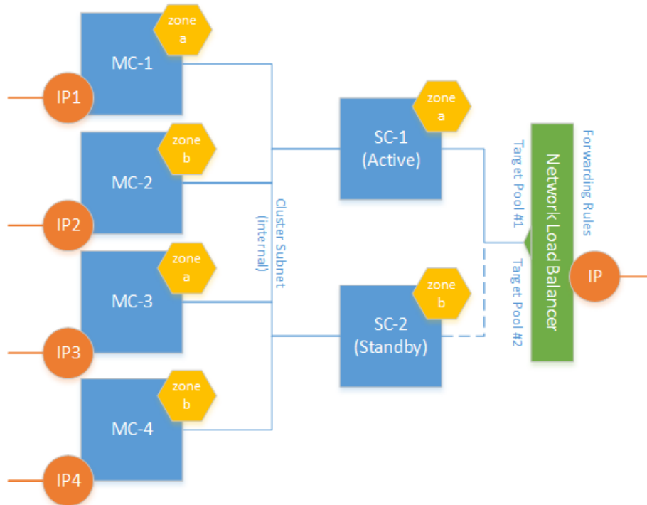
Figure 4-2: Mediant CE Deployment Topology (Google)
