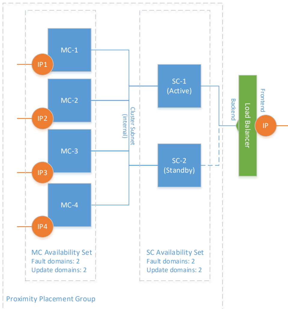
Figure 3-6: Mediant CE Deployment Topology (Azure)
