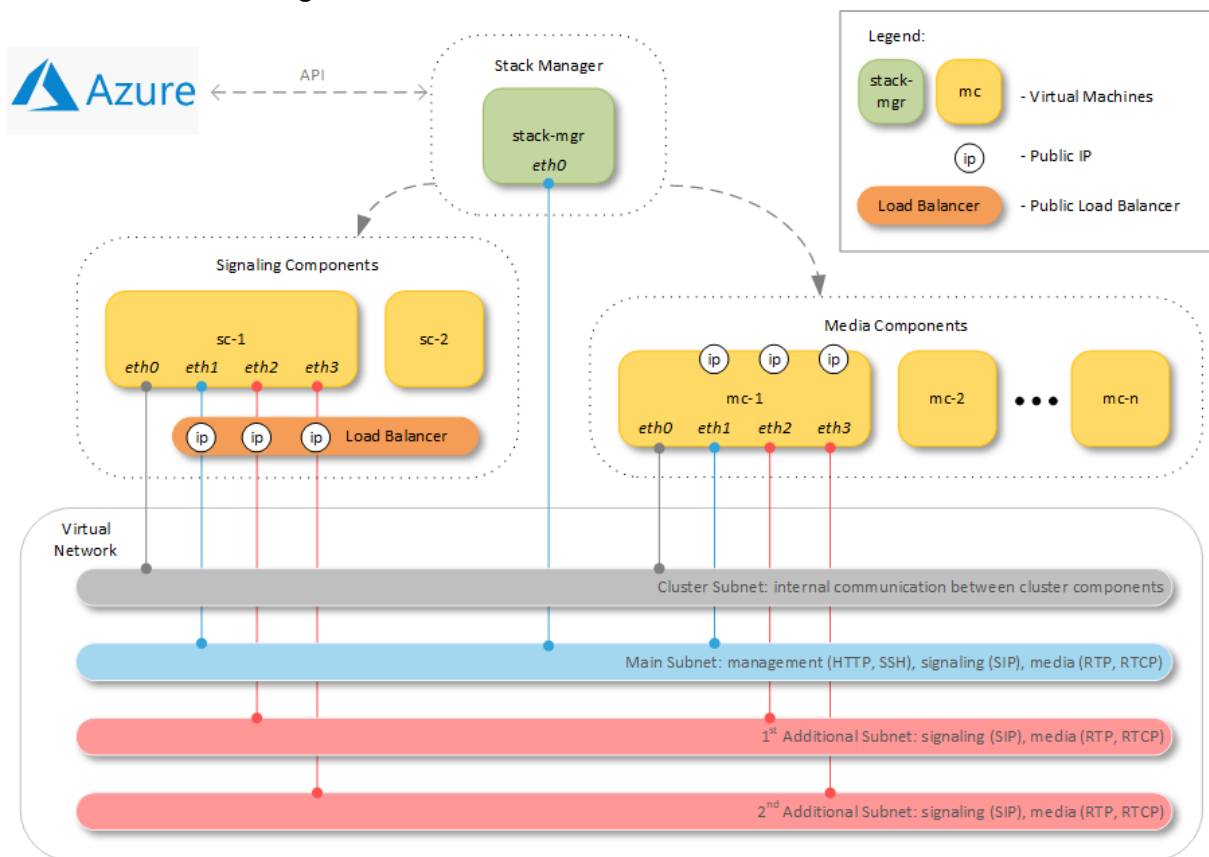
Figure 3-1: Mediant CE Network Architecture – Azure
