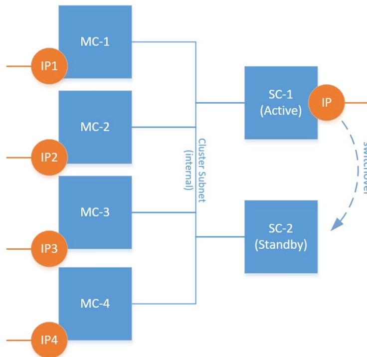
Figure 2-12: Mediant CE Deployment Topology (AWS)
