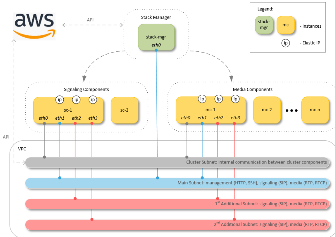
Figure 2-3: Mediant CE Network Architecture – AWS
