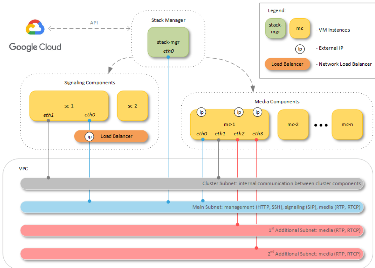
Figure 4-1: Mediant CE Network Architecture – Google Cloud
