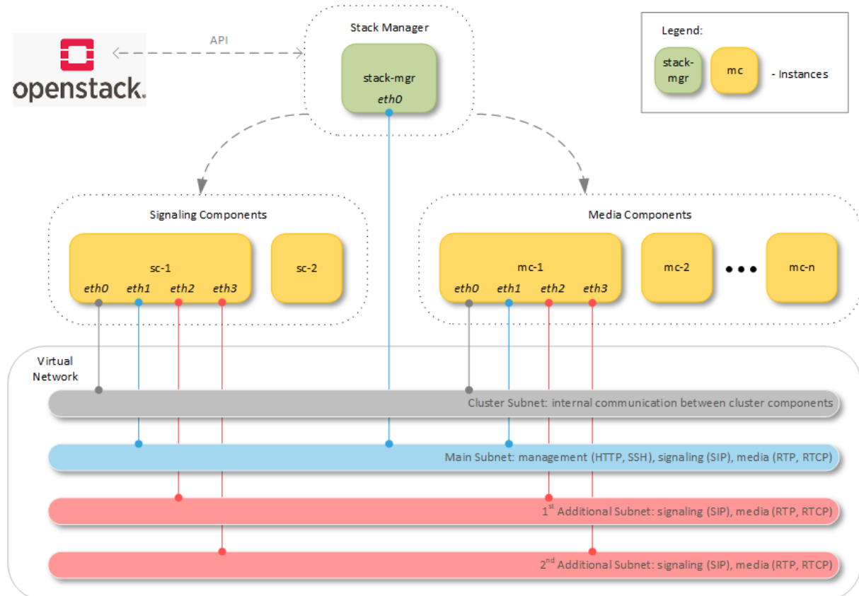
Figure 5-1: Mediant CE Network Architecture – OpenStack
