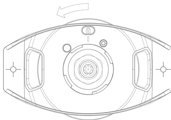
FIGURE 24: ROOF MOUNT INSTALLATION STEP 5 (LOCKED POSITION OF THE LT-300 GNSS RECEIVER)
