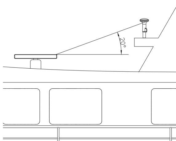
FIGURE 10: POLE MOUNT INSTALLATION STEP 3 (LOCATE AN APPROPRIATE LOCATION)
