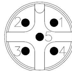
FIGURE 35: NMEA 2000 SCREW-IN CONNECTOR PIN NO.
