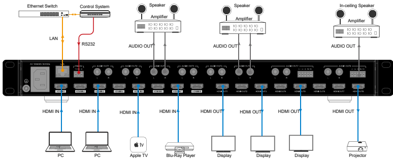
Application Diagram
