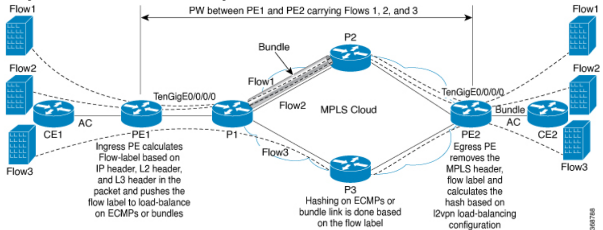
Figure 102: FAT PW with Two Flows Distributing over ECMPs and Bundle
