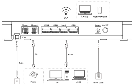
Figure 7-1 Entire Connection
